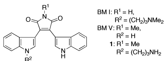
Figure 1. Structures of BM I, BM V, and 1 .
