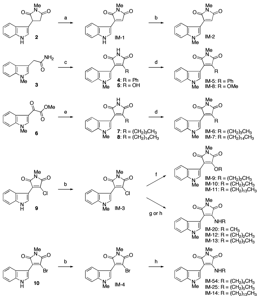
Scheme 1. Synthesis of indolylmaleimide derivatives. Reagents: (a) DDQ, dioxane (45%); (b) MeI, K 2 CO 3 , DMF (IM-2: 98%, IM-3: 88%, and IM-4: 95%); (c) PhCOCO 2 Et or (CO 2 Me) 2 , t -BuOK, DMF ( 4 : 88% and 5 : 90%); (d) MeI, NaH, DMF (IM-5: 97%, IM-6: 84%, IM-7: 90%, and IM-8: 16%); (e) RCH 2 CONH 2 , t -BuOK, DMF ( 7 : 77% and 8 : 61%); (f) ROH, NaH, THF (IM-9: 90%, IM-10: 91%, and IM-11: 93%); (g) 40%MeNH 2 aq/THF (2/1) (IM-20: 28%); (h) RNH 2 , CH 2 Cl 2 (IM-12: 82%, IM-13: 76%, and IM-14: 88%) or THF (IM-54: 59% and IM-25: 83%).
