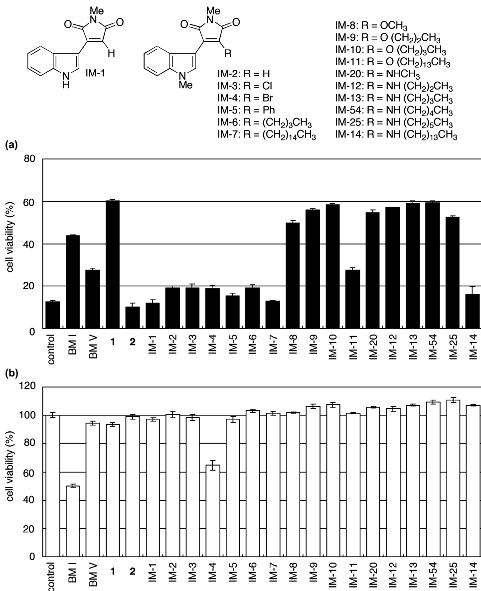
Figure 2. Structure and activities of various indolylmaleimide derivatives. (a) Cell death inhibition: viability of HL60 cells treated with H 2 O 2 (100 μM, 3 h) in the absence (control) or the presence of 3 μM indolylmaleimide derivative. (b) Cytotoxicity: viability of HL60 cells treated with 10 μM indolylmaleimide derivative.
